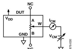
Figure 32. Common-Mode Leakage Current
