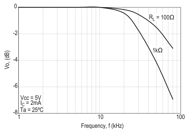
Figure 19 Frequency Response
