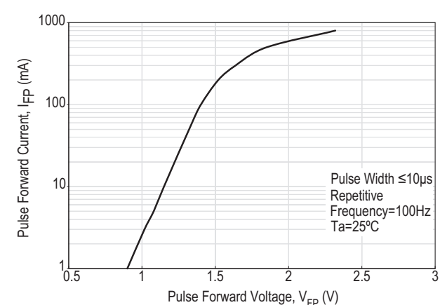
Figure 8 Pulse Forward Current vs. Pulse Forward Voltage
