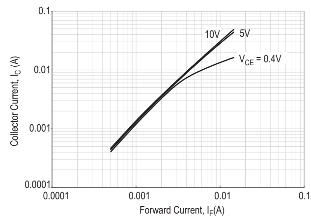
Figure 11 Collector Current vs. Forward Current
