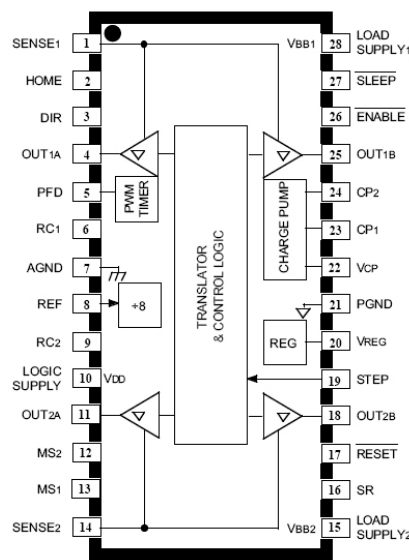
LP Package, 28-Pin TSSOP Pinout Digram
