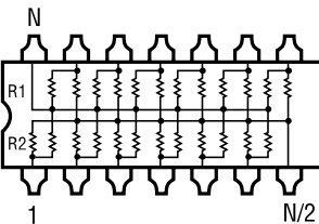
-5 Circuit - Dual Terminator
