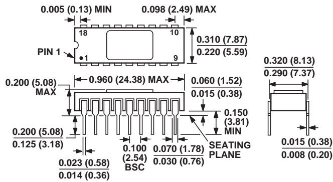
CONTROLLING DIMENSIONS ARE IN INCHES; MILLIMETER DIMENSIONS (IN PARENTHESES) ARE ROUNDED-OFF INCH EQUIVALENTS FOR REFERENCE ONLY AND ARE NOT APPROPRIATE FOR USE IN DESIGN.
