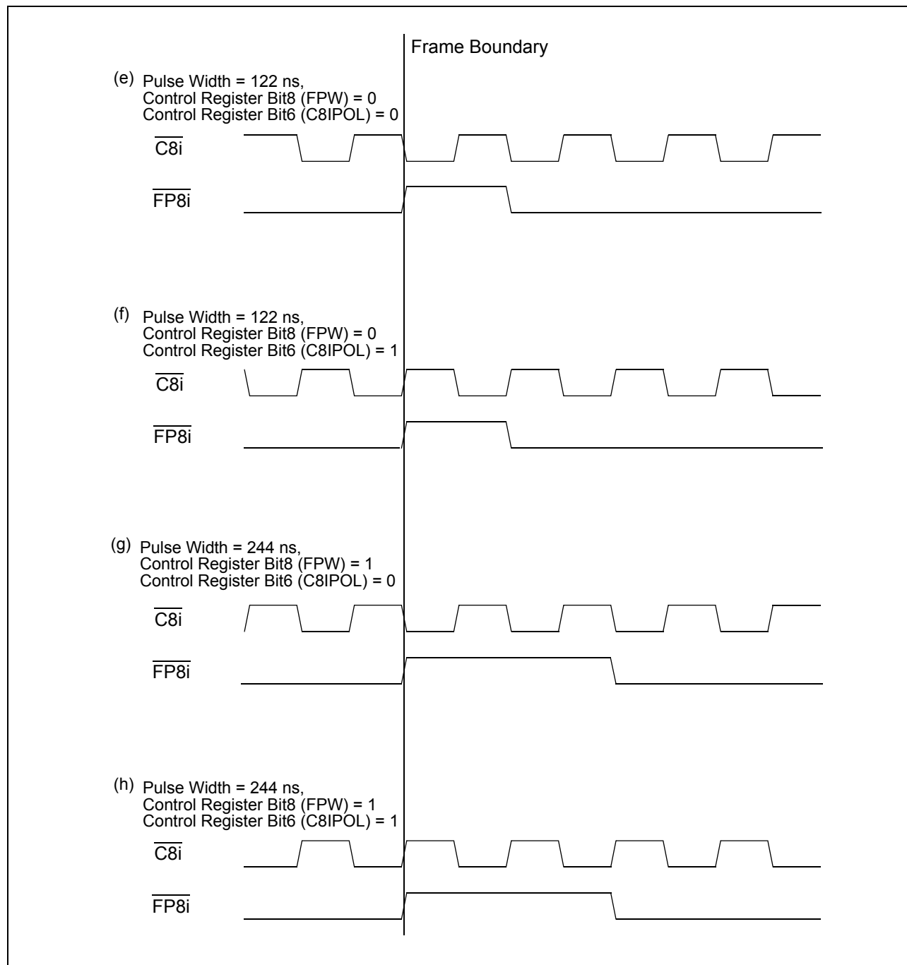
Figure 23 - Frame Boundary Conditions, GCI-Bus Operation
