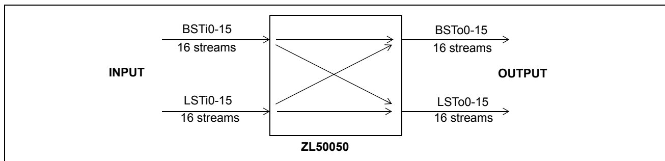
Figure 3 - 8,192 x 8,192 Channels (16 Mbps), Unidirectional Switching
