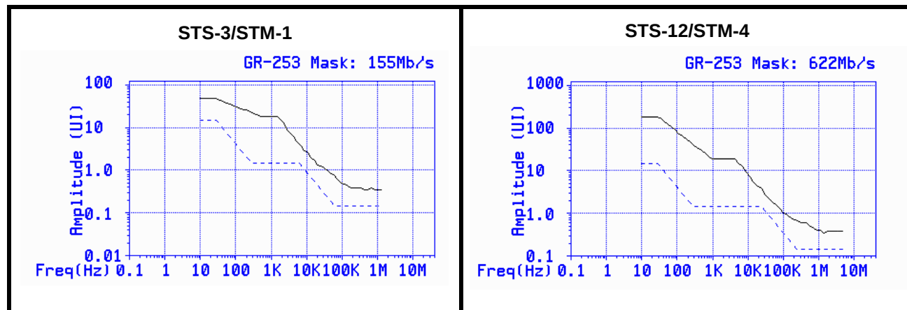
FIGURE 24. XRT91L30 MEASURED JITTER TOLERANCE WITH 77.76MHz REFERENCE CLOCK
