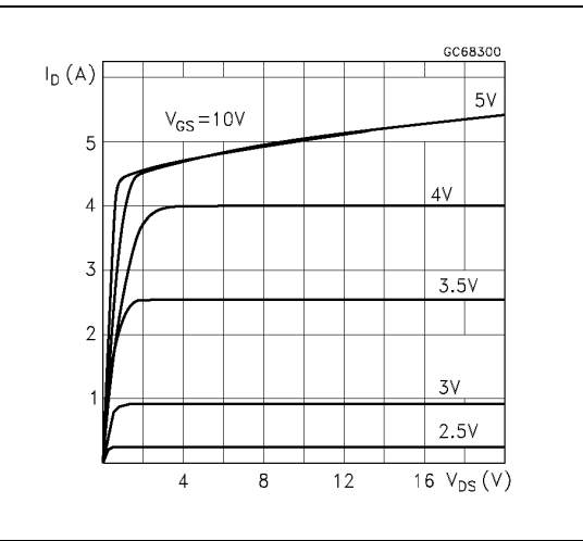
Figure 26. Output characteristics
