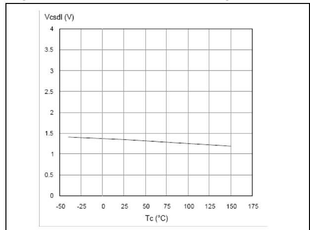
Figure 25. CS_DIS low level voltage
