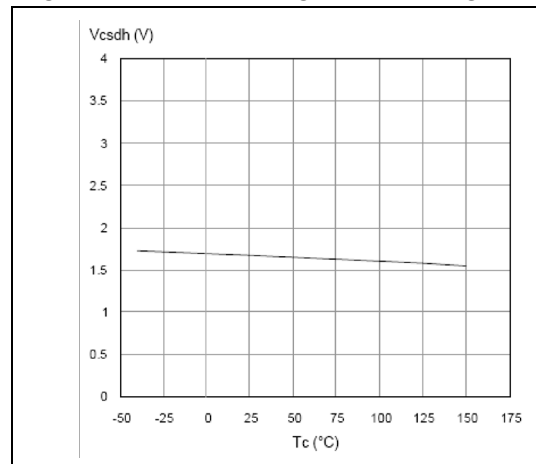
Figure 23. CS_DIS high level voltage
