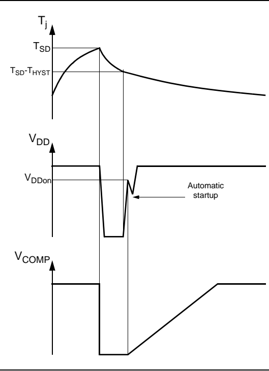
Figure 7. Thermal shutdown
