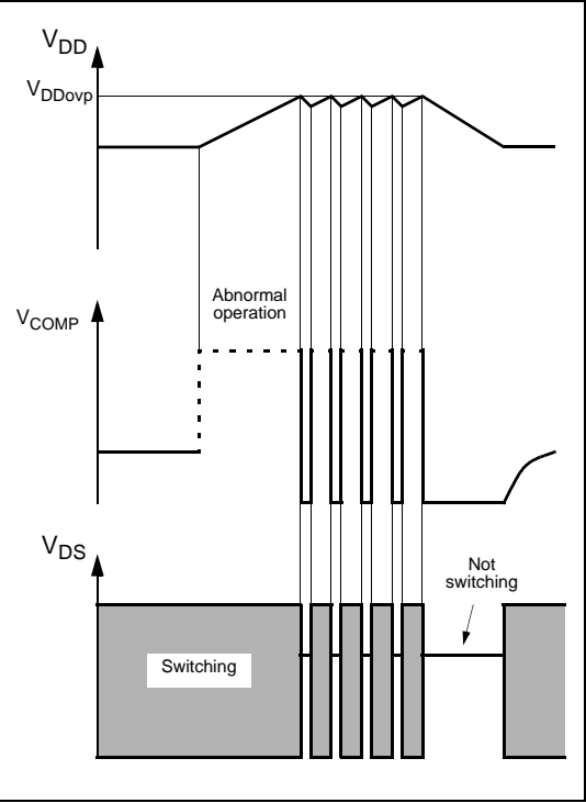
Figure 8. Overvoltage event
