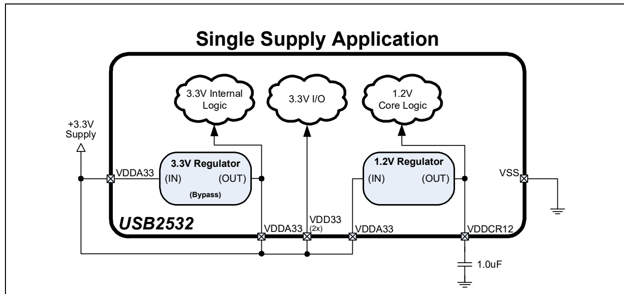
FIGURE 4-1: POWER CONNECTIONS
