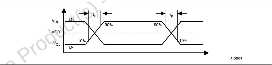
Figure 45. USB data signal timing and voltage levels
