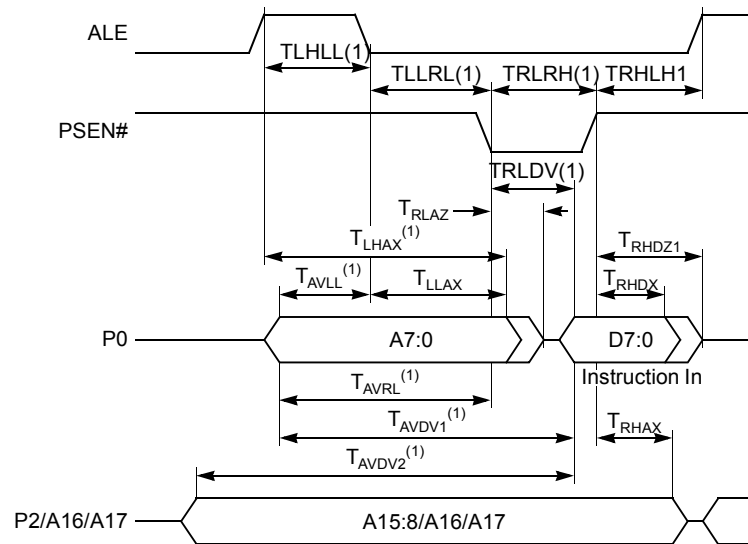
Waveforms in Non-Page Mode
