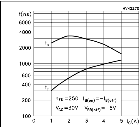
Figure 14. Resistive load switching time (NPN, off)
