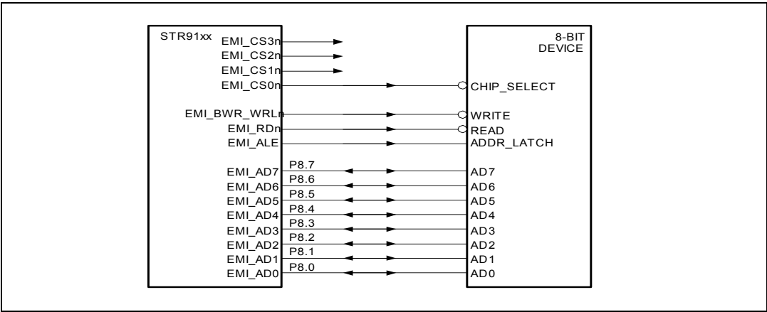
Figure 5. EMI 8-bit multiplexed connection example
