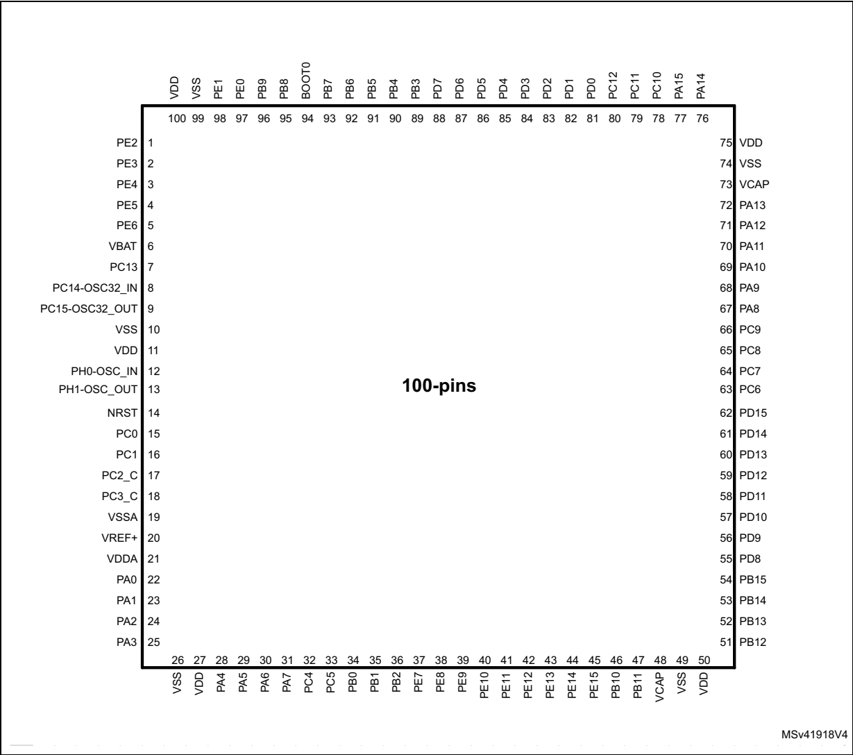
Figure 4. LQFP100 pinout
