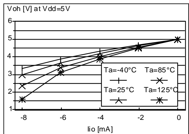
Figure 82. Typical V_{OH} at V_{DD}=5\text{V}
