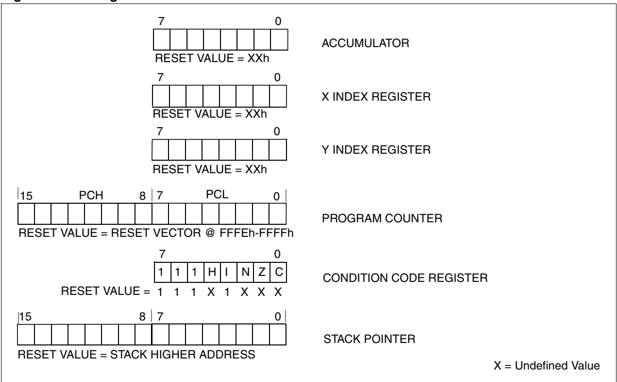
Figure 6. CPU Registers
