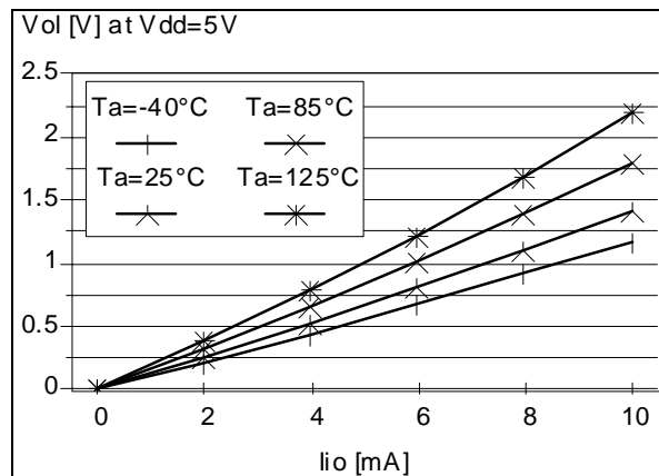
Figure 81. Typical V_{OL} at V_{DD}=5\text{V} (high-sink)
