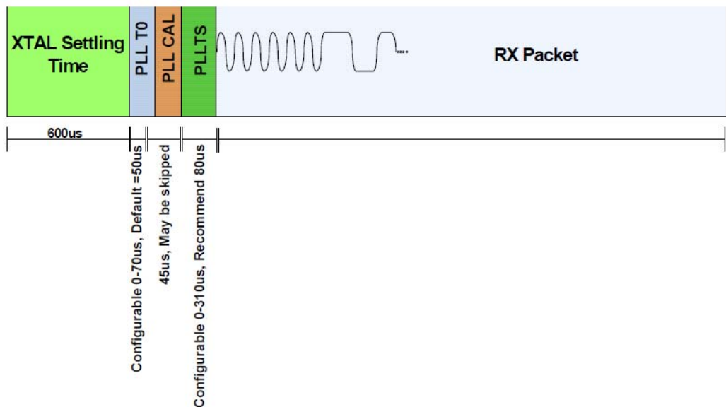
Figure 7. RX Timing
