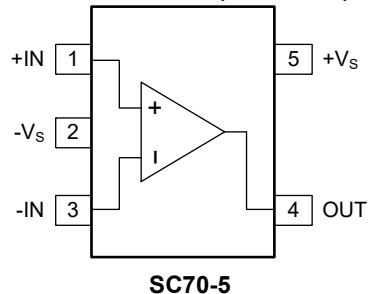
SGM8049-1BXC5G (TOP VIEW)
