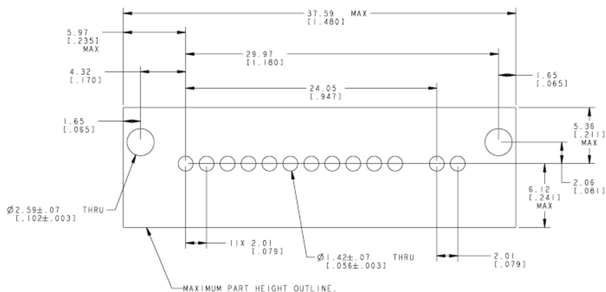
Recommended Pad Layout
