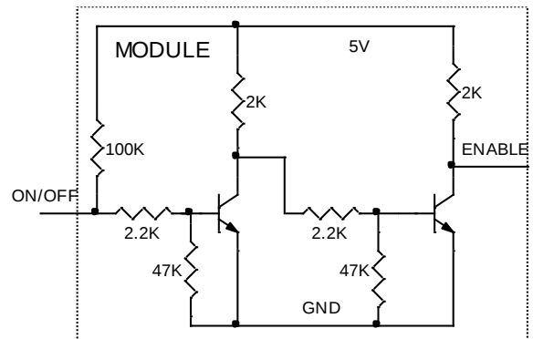
Figure 41. Remote On/Off Implementation.
