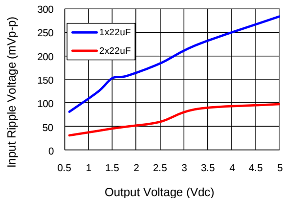
Figure 40. Input ripple voltage for various output voltages with 1x22 μF or 2x22 μF ceramic capacitors at the input (40A load). Input voltage is 12V.
