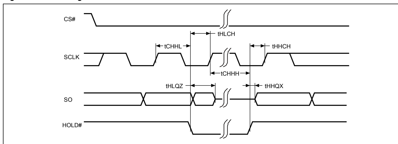
Figure 4. Hold Timing
