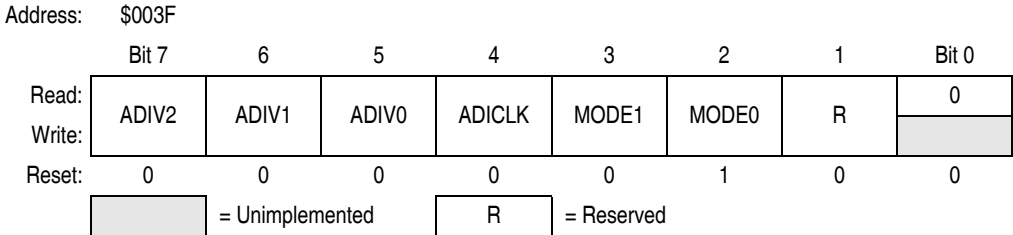
Figure 3-9. ADC Clock Register (ADCLK)
