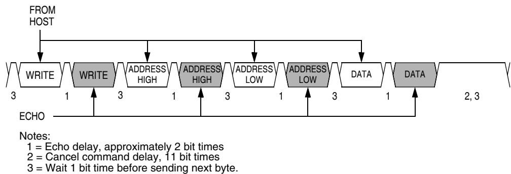
Figure 20-15. Write Transaction
