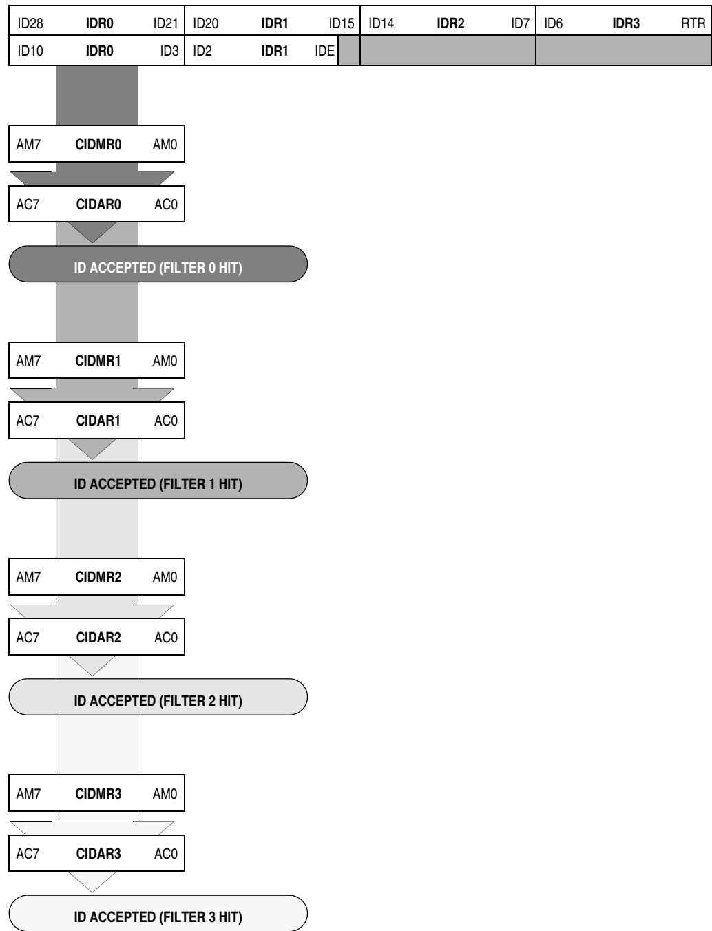
Figure 12-6. Quaduple 8-Bit Maskable Acceptance Filters
