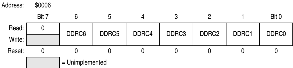
Figure 13-10. Data Direction Register C (DDRC)
