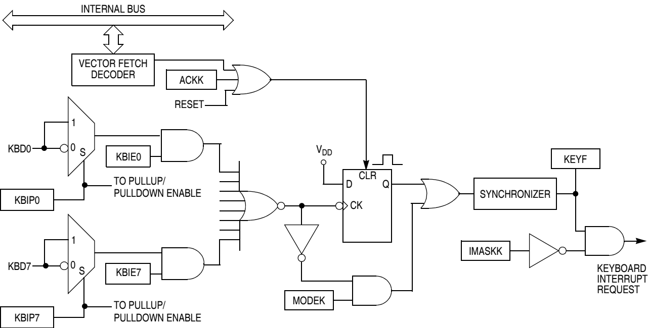
Figure 9-2. Keyboard Module Block Diagram
