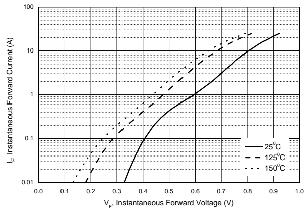
Figure 1. Typical Forward Voltage Per Diode
