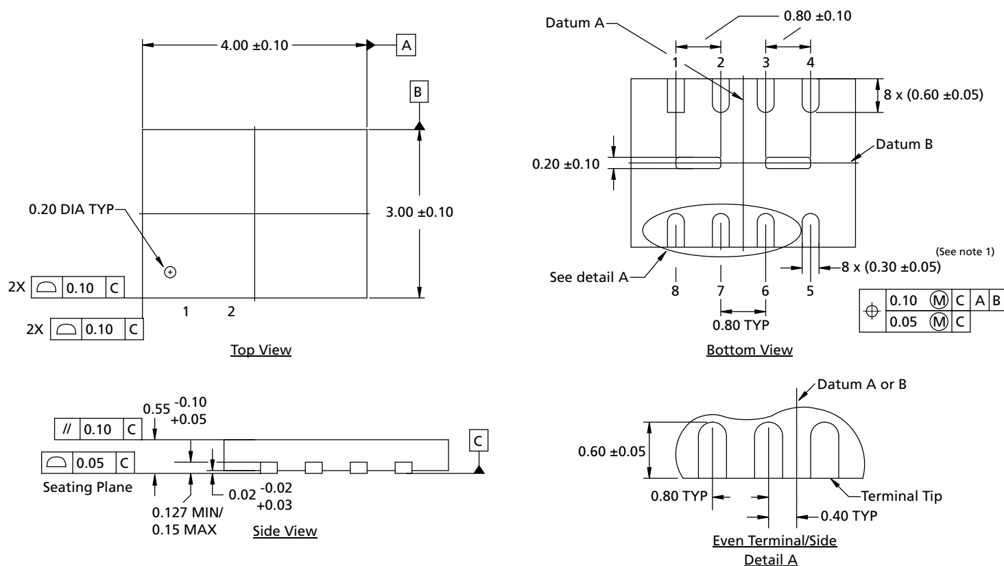
Figure 32: UDFPN8 (MLP8) 4mm x 3mm
