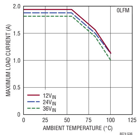
Derating, V_{OUT} = 1\text{V} , DC2753A Demo Board
