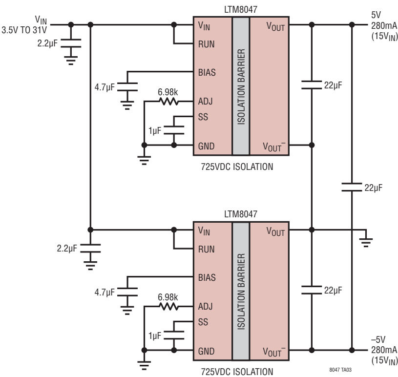
Use Two LTM8047 Flyback Converters to Generate ±5V
