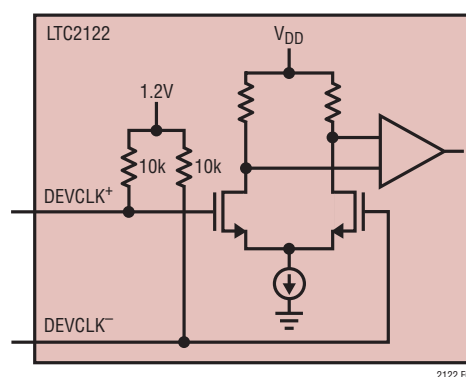
Figure 8. Equivalent DEVCLK Input Circuit
