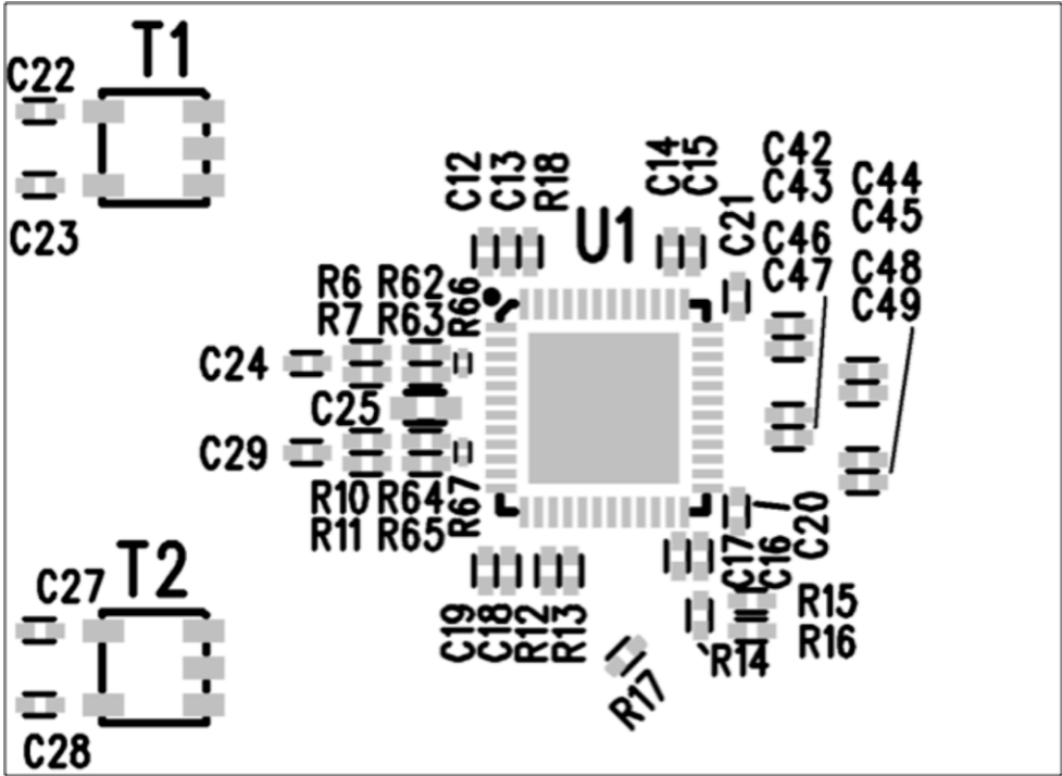
Silkscreen Top
