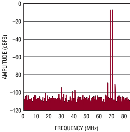
64k Point 2-Tone FFT, f_{IN} = 71\text{MHz} and 69\text{MHz} , -7dBFS, 170Msps
