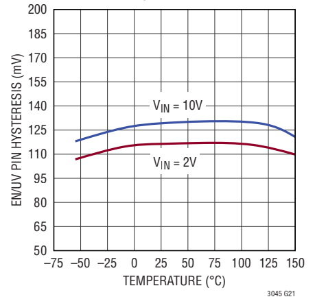
EN/UV Pin Hysteresis
