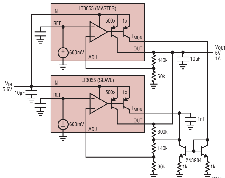
Figure 10. Paralleling Devices
