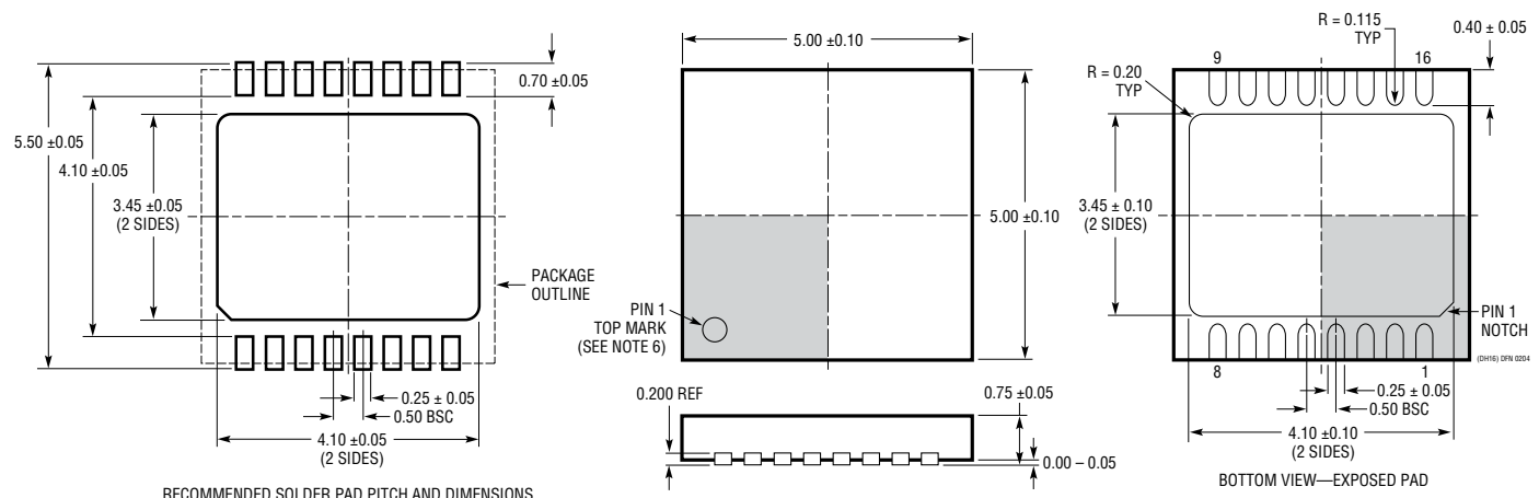
DH Package 16-Lead Plastic DFN (5mm \times 5mm) (Reference LTC DWG # 05-08-1709)
