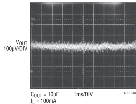
LT1761-5 10Hz to 100kHz Output Noise C_{BYP} = 0.01\mu F
