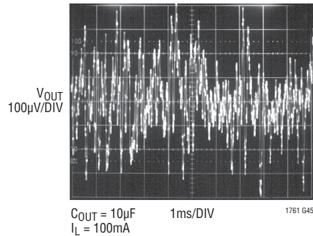
LT1761-5 10Hz to 100kHz Output Noise C_{BYP} = 0pF
