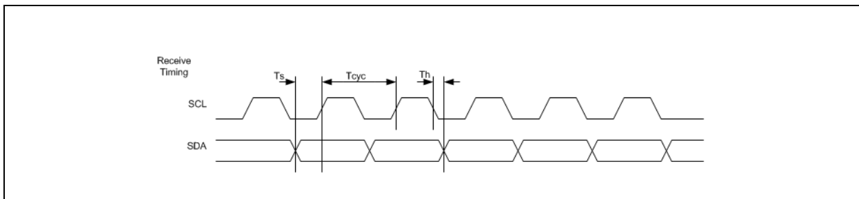
FIGURE 7-9: I 2 C INPUT TIMING
