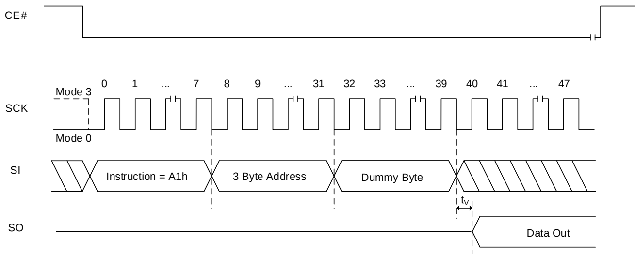
Figure 8.25 RDUID Operation
