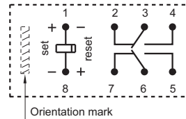
Reset condition
