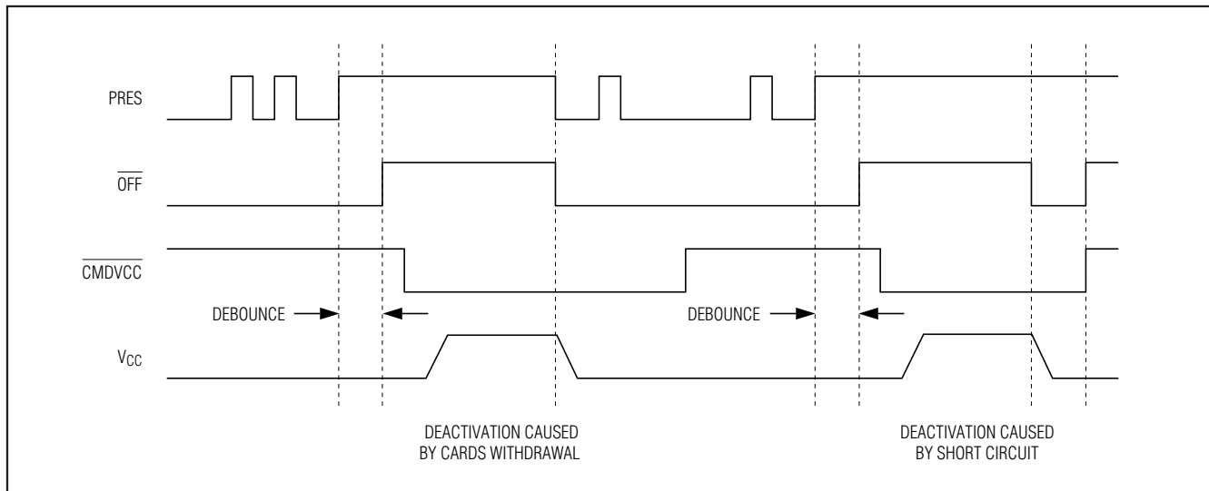
Figure 6. Behavior of PRES, \overline{\text{OFF}} , \overline{\text{CMDVCC}} , and \text{V}_{\text{CC}}
