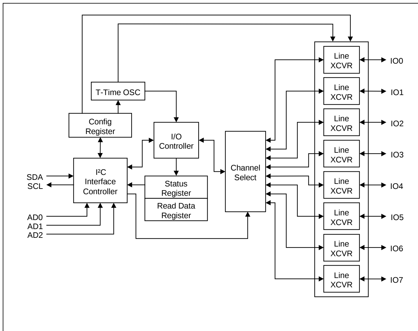
Figure 1. Block Diagram
