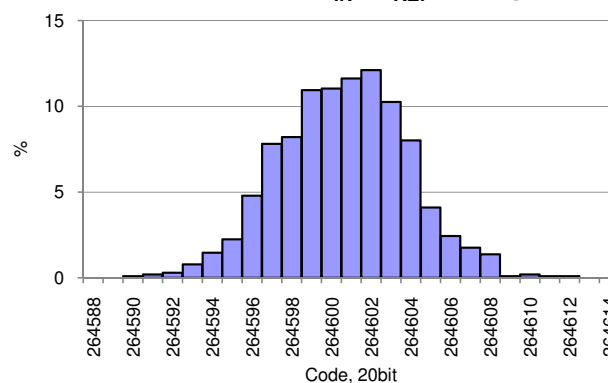
Figure 11-34. Delta-sigma ADC Noise Histogram, 1000 Samples, 20-Bit, 187 sps, Ext Ref, V_{IN} = V_{REF}/2 , Range = \pm 1.024 V
