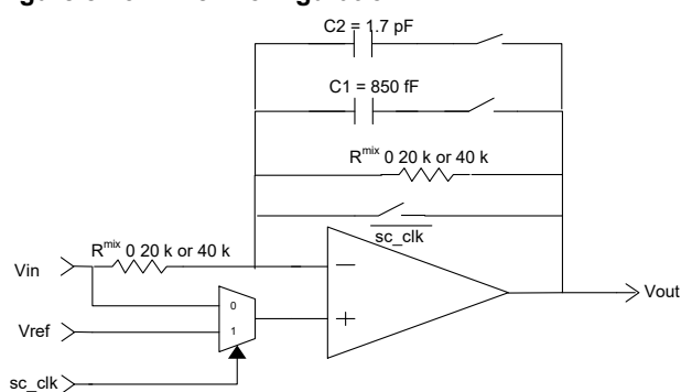
Figure 8-13. Mixer Configuration
