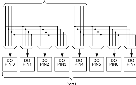
Figure 7-12. I/O Pin Output Connectivity
