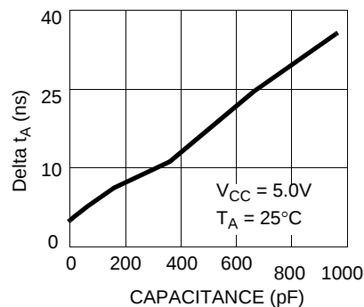
TYPICAL t_A CHANGE vs. OUTPUT LOADING
