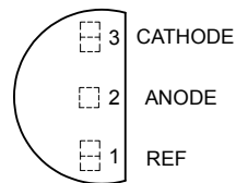
Figure 2. Pin Configuration of AZ431-B (Top View)
