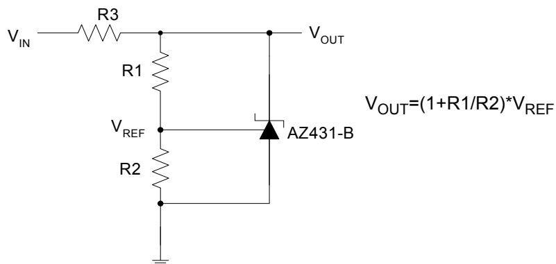
Figure 17. Shunt Regulator
