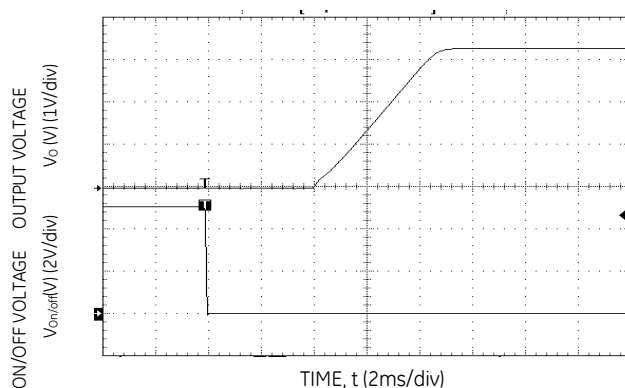
Figure 15. Typical Start-Up Using Remote On/Off with Low-ESR external capacitors ( 7 \times 150\text{ }\mu\text{F} Polymer) ( V_{in} = 5.0\text{Vdc} , V_o = 3.3\text{Vdc} , I_o = 3\text{A} , C_o = 1050\text{ }\mu\text{F} ).
