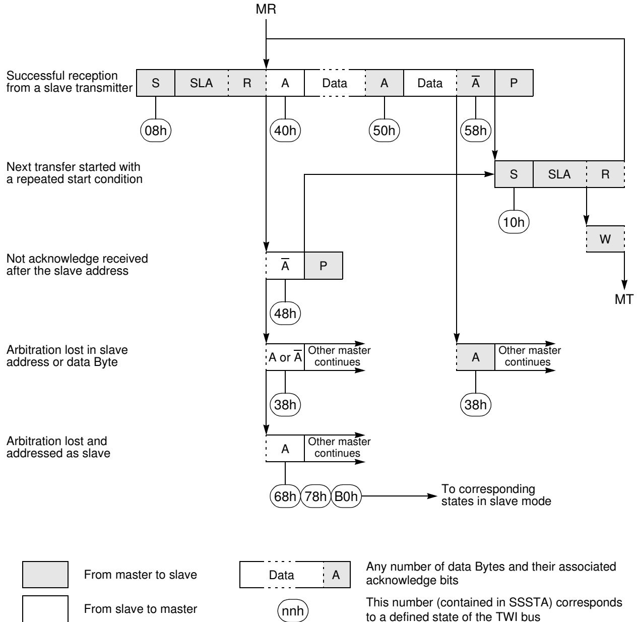
Figure 20-4. Format and States in the Master Receiver Mode
