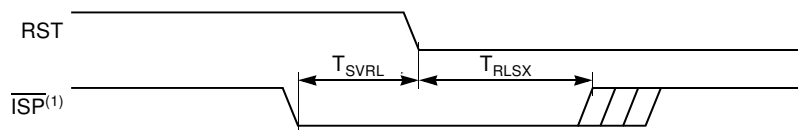
Figure 23-23. FLASH Memory - ISP Waveforms
