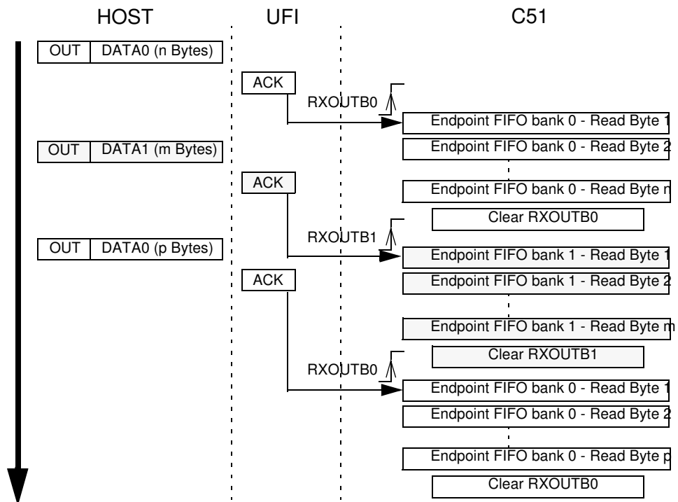
Figure 15-10. Bulk/Interrupt OUT Transactions in Ping-pong Mode
