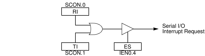
Figure 18-16. Serial I/O Interrupt System
