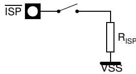
Figure 23-8. ISP Pull-Down Connection
