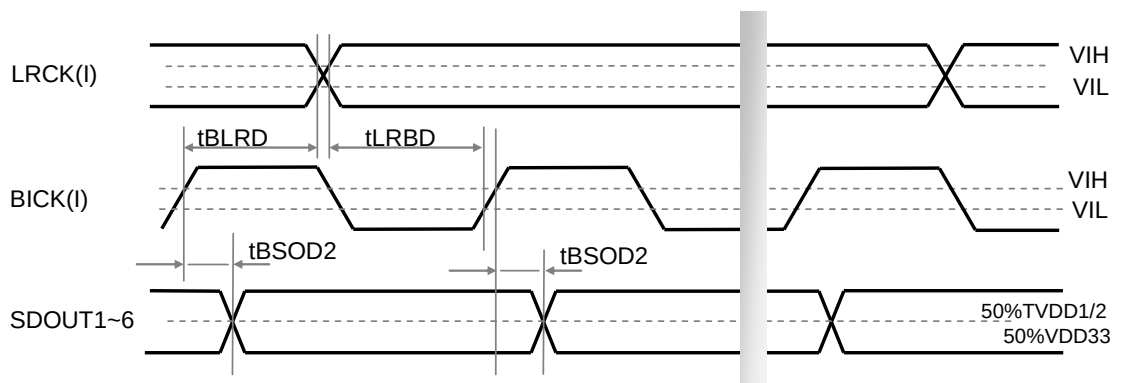
Figure 9. Serial Interface Output Timing in Slave Mode (SDOPHx bit = "1")
