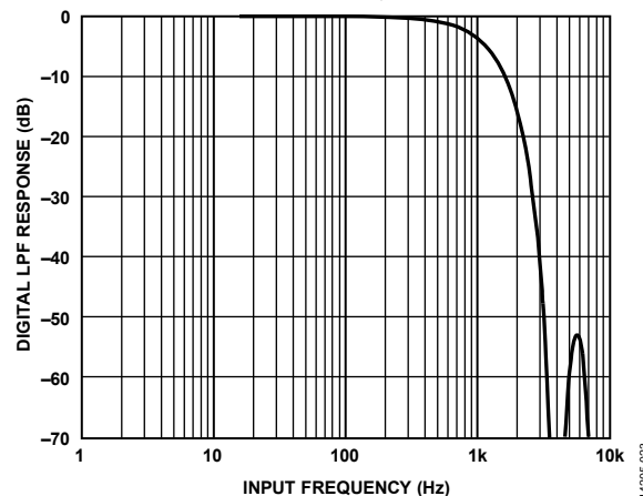
Figure 61. ADXL355 Digital LPF Response for 4 kHz ODR
