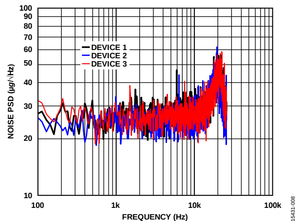
Figure 8. ADXL1002 Noise Power Spectral Density (PSD)
