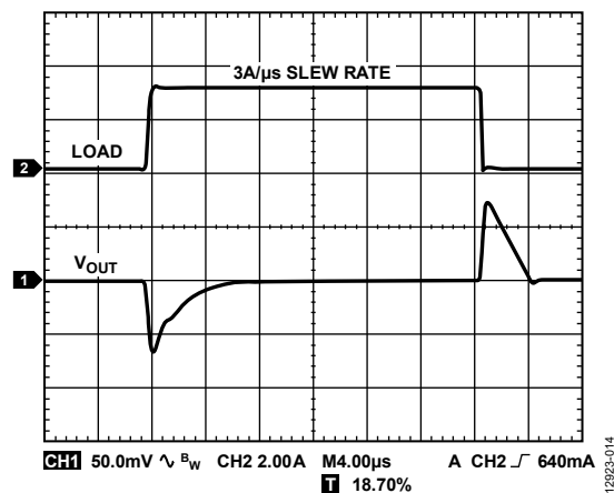
Figure 14. Load Transient Response, C_{OUT} = 10 μF, V_{IN} = 1.8 V, V_{OUT} = 1.3 V
