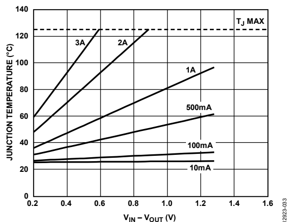
Figure 35. 6400 mm 2 of PCB Copper, T_A = 25^\circ\text{C}
