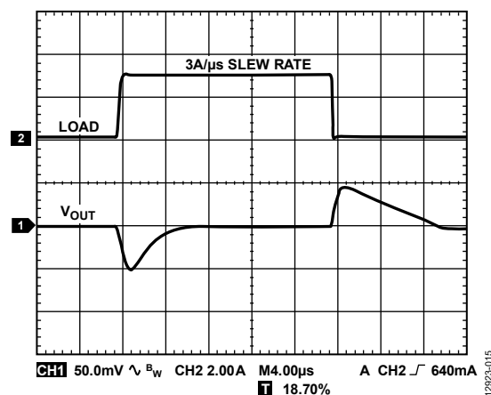
Figure 15. Load Transient Response, C_{OUT} = 47 μF, V_{IN} = 1.8 V, V_{OUT} = 1.3 V
