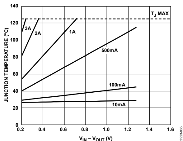
Figure 37. 25 mm 2 of PCB Copper, T_A = 25^\circ\text{C}
