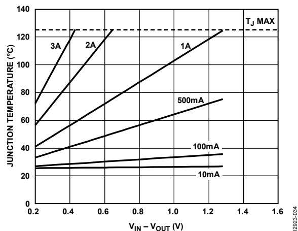
Figure 36. 500 mm 2 of PCB Copper, T_A = 25^\circ\text{C}
