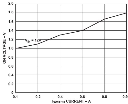
Figure 3. Switch ON Voltage vs. I_{\text{SWITCH}} Current In Step-Down Mode
