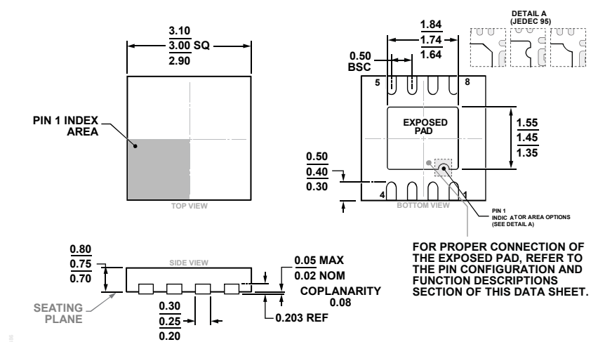
Figure 65. 8-Lead Lead Frame Chip Scale Package [LFCSPP] 3 mm × 3 mm Body and 0.75 mm Package Height (CP-8-13)
