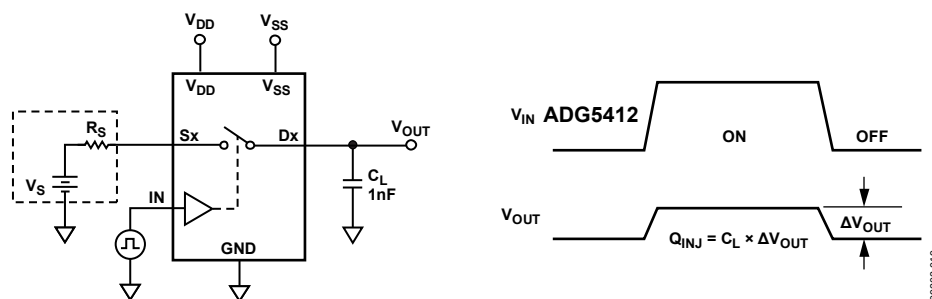
Figure 32. Charge Injection
