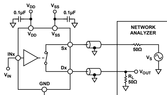
Figure 29. Bandwidth
