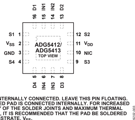
Figure 3. LFCSP Pin Configuration
