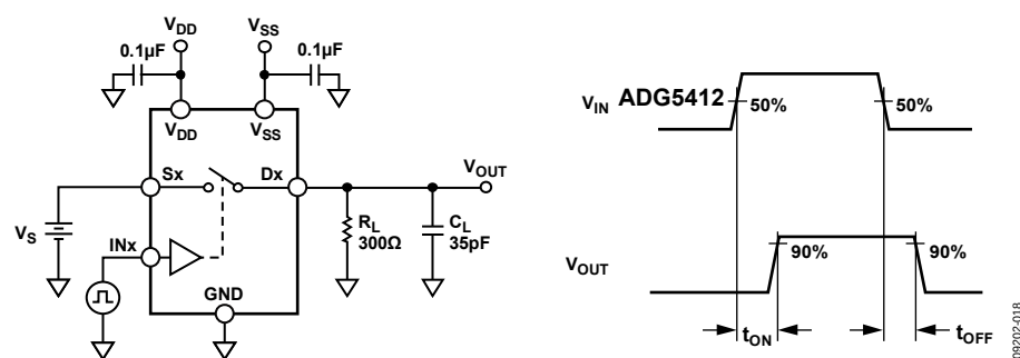
Figure 31. Switching Times
