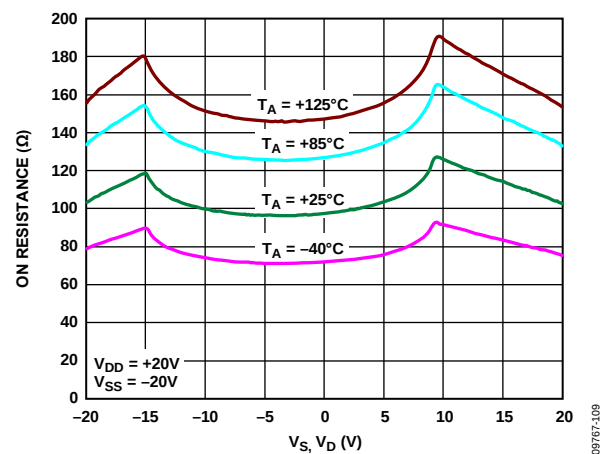
Figure 9. R_{ON} as a Function of V_S, V_D for Different Temperatures, \pm 20\text{ V} Dual Supply
