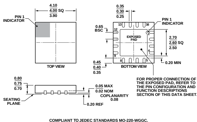
Figure 34. 16-Lead Lead Frame Chip Scale Package [LFCSP_WQ] 4 mm × 4 mm Body, Very Very Thin Quad (CP-16-17)
