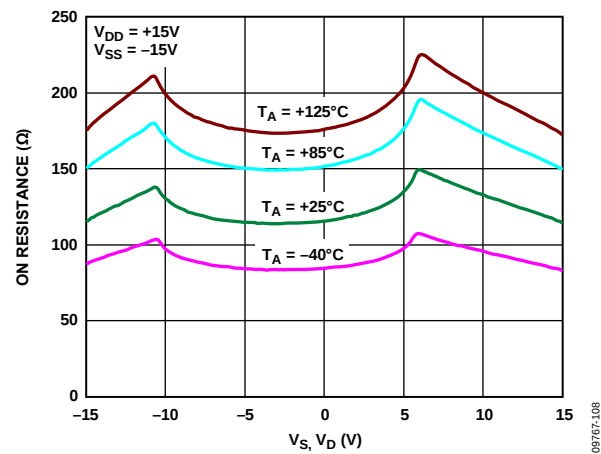
Figure 8. R_{ON} as a Function of V_S, V_D for Different Temperatures, \pm 15\text{ V} Dual Supply
