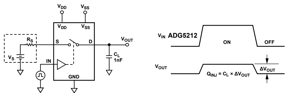
Figure 31. Charge Injection
